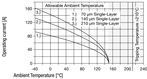
Derating Curve without Shunt
