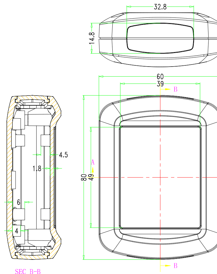
SEC B-B
