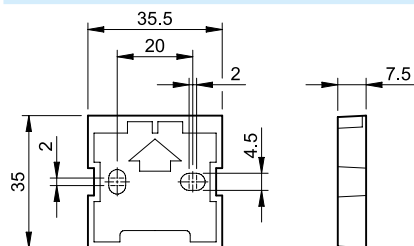
Adaptor for panel mounting, 35 mm wide
